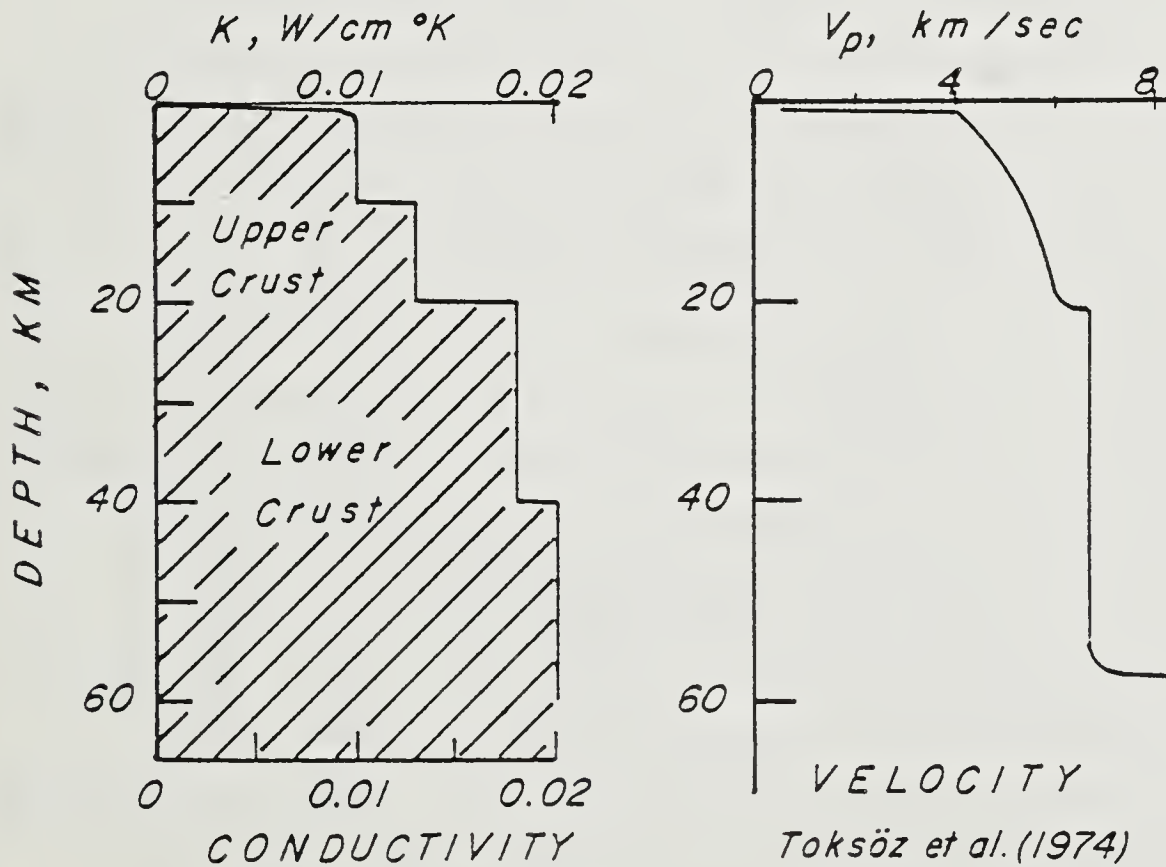
Top: Thermal conductivity versus porosity from laboratory measurements of returned lunar samples as summarized in Horai and Winkler (1976). Bottom: Inferred crustal thermal conductivity profile (left) based on a correlation of porosity and the seismic profile (right) of Toksöz et al. (1974)
